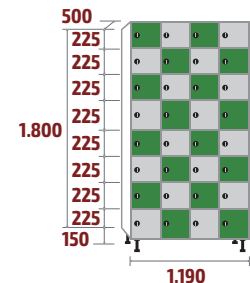
FZ-30/4 COD: 53173 201kg · 1,07m 3
